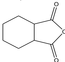
monomer 1
